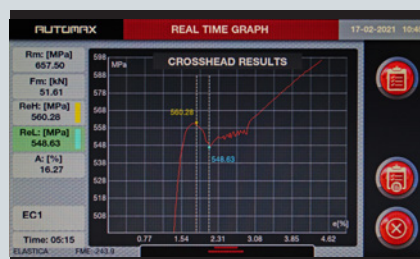
Tensile test results
