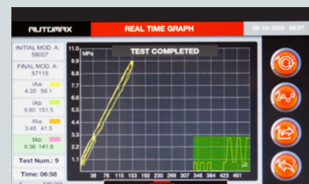
Elastic Modulus test results
